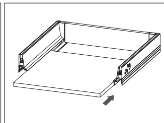
Assembly - Bottom
